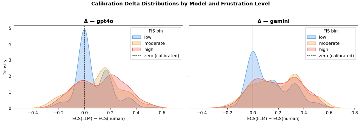
Figure 1: Calibration Delta Distributions by Model and Frustration Level.
